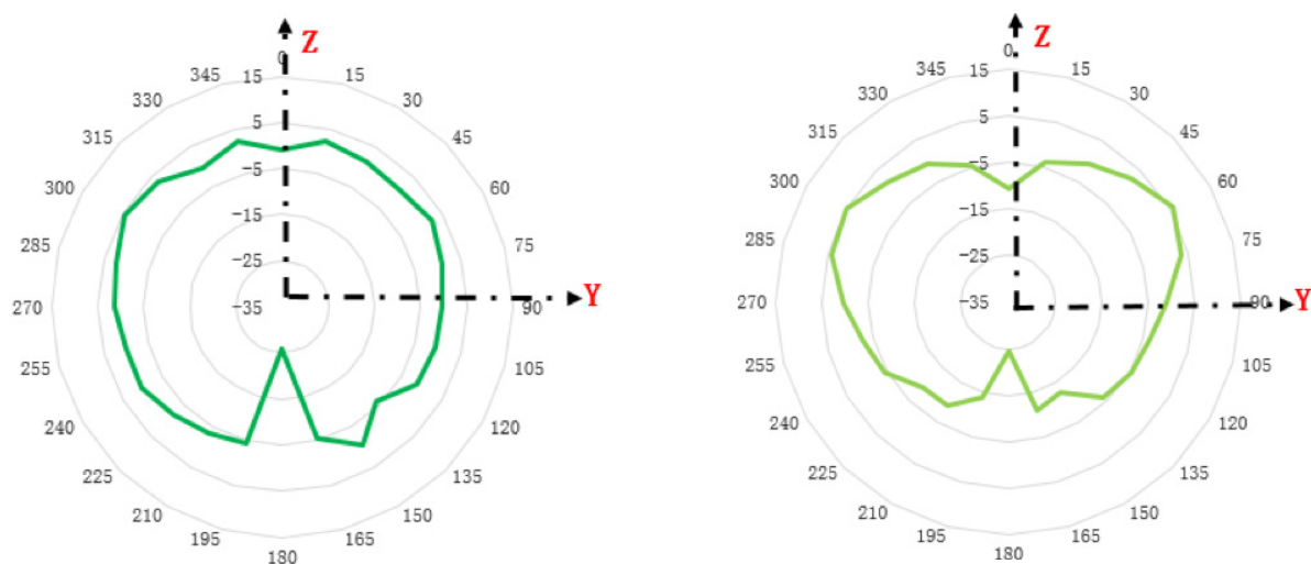
Elevation plane (side view, 90 degrees angle)
